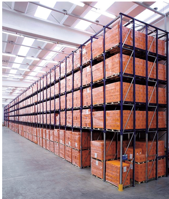
Figura 1-2: Scaffalatura porta pallet ad accumulo (Drive In, Drive Through)
